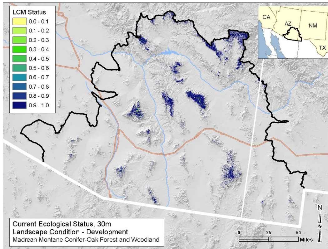
Figure D-44. Scores for three indicators for Madrean Montane Conifer-Oak Forest and Woodland: development indicator (first map), fire regime departure indicator (second map), and invasive species indicator (third map) for each 30m pixel. At the ecoregion scale, many development features are not readily visible (i.e. secondary roads or highways, railroads, small agricultural fields). Yellow (equivalent to 0) indicates high impacts from the CA, dark blue (equivalent to 1) indicates little to no impact from the CA. Only 3 classes of fire regime condition are scored: no to little departure (dark blue), moderate departure and severe departure (lighter blues). For the invasives indicator results, higher cover of mesquite or invasive exotics will score between .4 and .6 (light greens), while lower cover scores between .6 and .8 (light blues).
