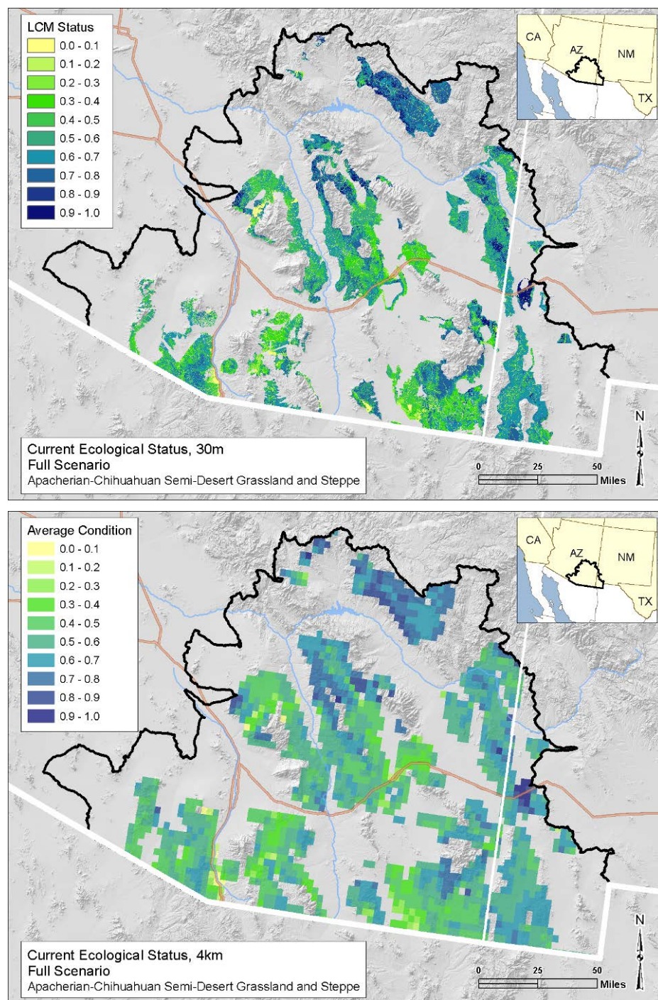
Figure D-13. Overall ecological status scores for Apacherian-Chihuahuan Semi-Desert Grassland and Steppe for all indicators combined (development, fire regime and invasives) for each 30m pixel (top) and 4km grid cells (bottom). The score for each 4km cell is an average of all 30m pixels that are scored for the CE. Yellow scores (equivalent to 0) indicate high impacts from the CAs, dark blue (equivalent to 1) indicate little to no impact from the CAs.
